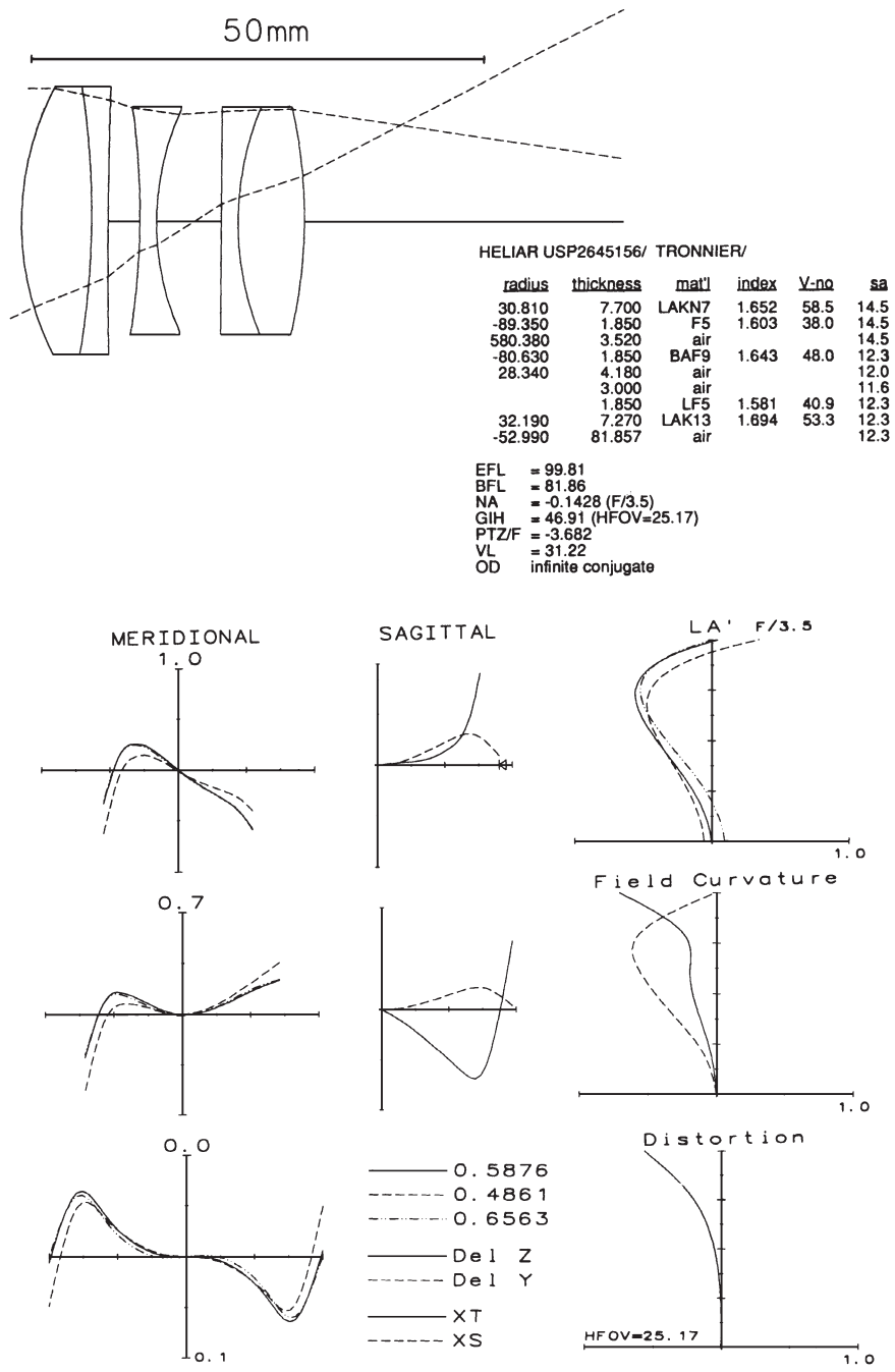
Figure 14.18 The Heliar form has doublets front and rear, gaining the advantage of a roughly symmetrical construction. Just as the Tessar is better than the Cooke triplet, the Heliar is better than the Tessar.
